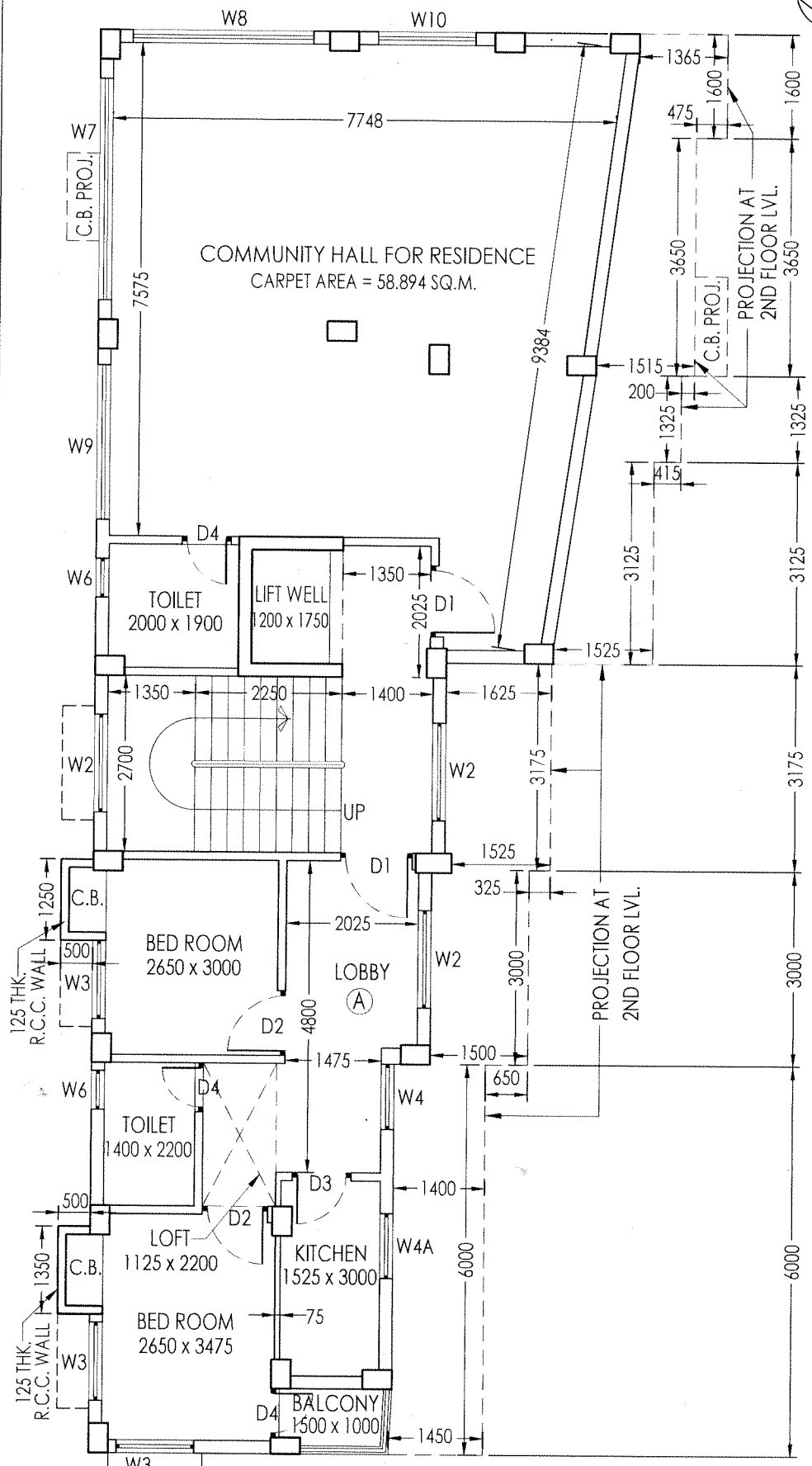
1ST FLOOR PLAN REAR BLOCK
