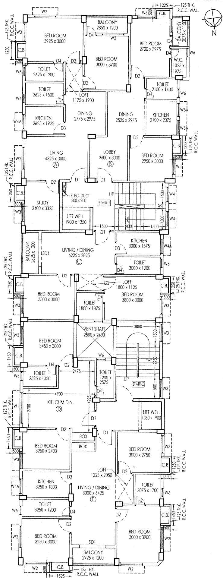
2ND TO 6TH FLOOR PLAN FRONT BLOCK
