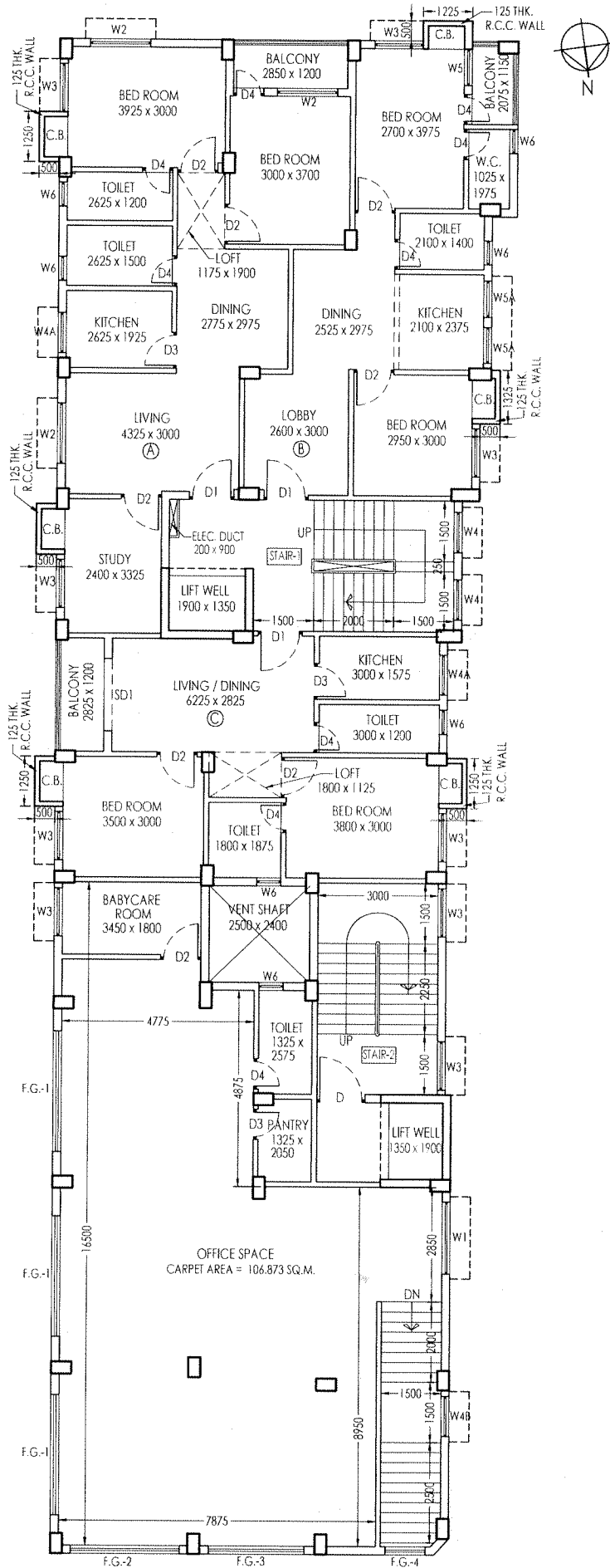
1ST FLOOR PLAN FRONT BLOCK
