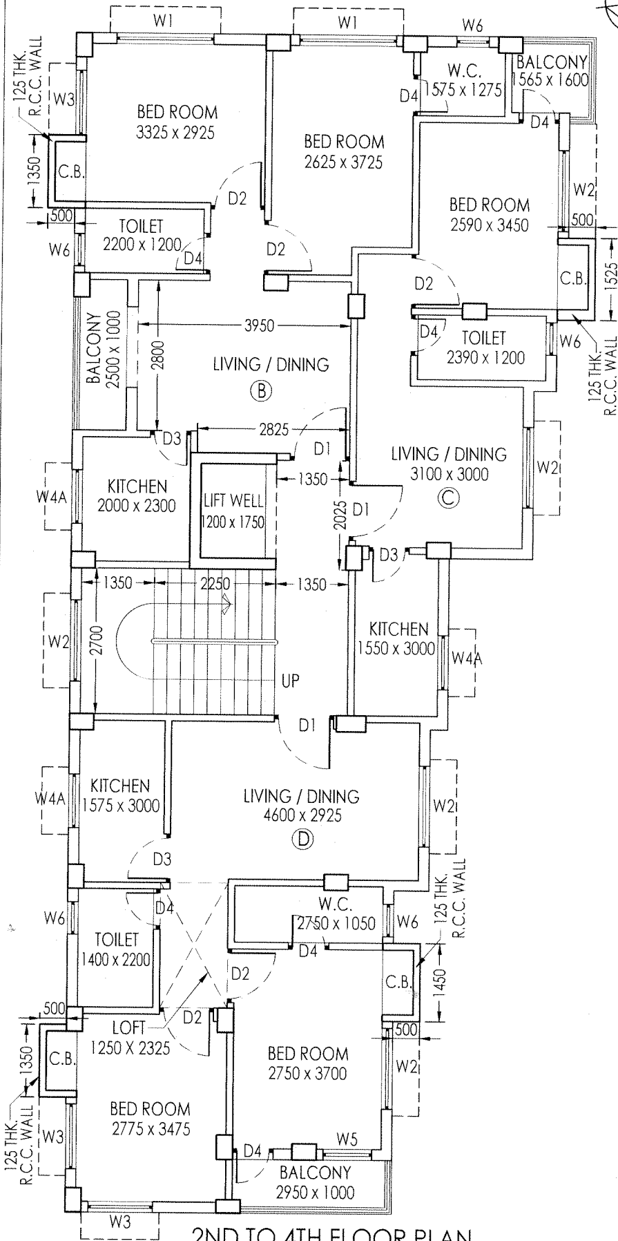
2ND TO 4TH FLOOR PLAN REAR BLOCK
